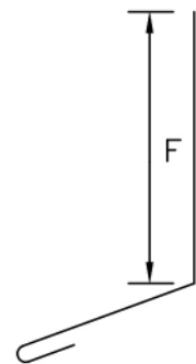
SILL FLASHING
