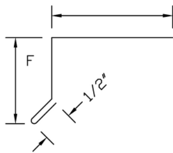
GABLE FLASHING
