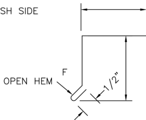
SILL FLASHING
