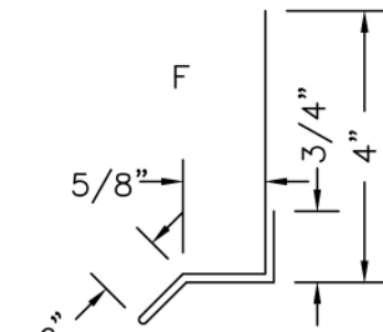
DRIP FLASHING
