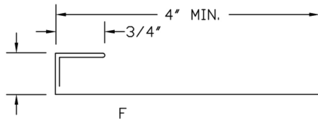
CHANNEL CLOSURE
