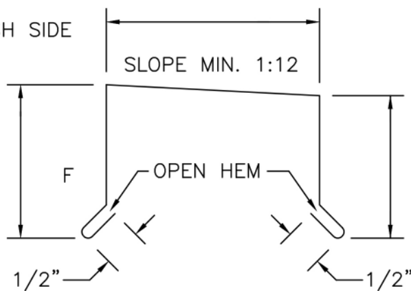
CAP FLASHING
